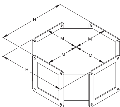
Cross Fitting
