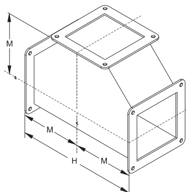
Tee Fitting
