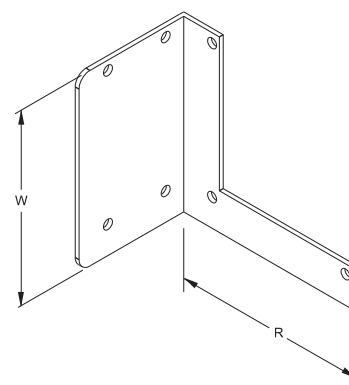
Bracket Hanger
