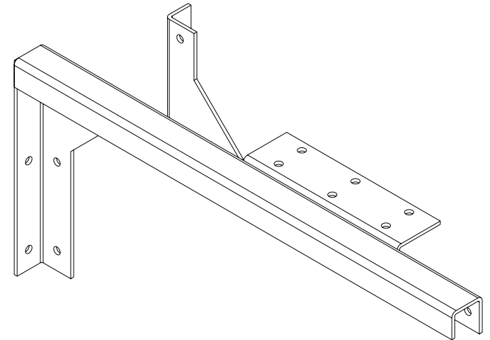
ISOMETRIC VIEW
