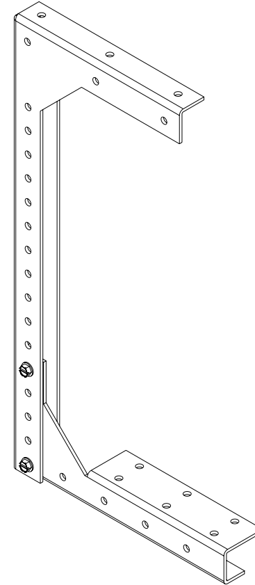
ISOMETRIC VIEW
