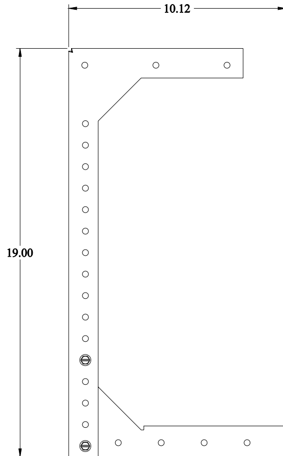
FRONT VIEW
