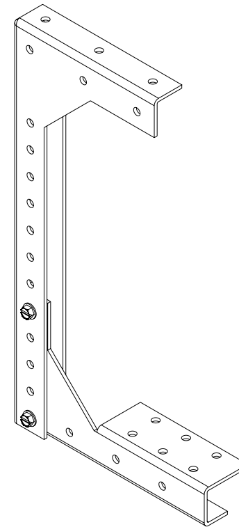
ISOMETRIC VIEW
