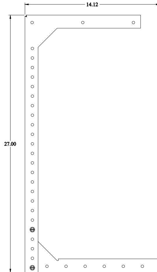
FRONT VIEW
