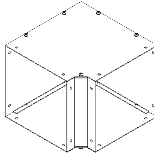
ISOMETRIC VIEW
