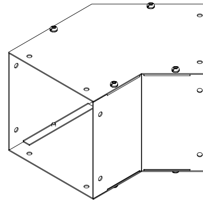
ISOMETRIC VIEW
