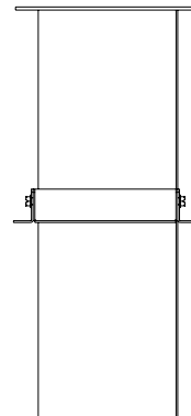
BOTTOM VIEW
