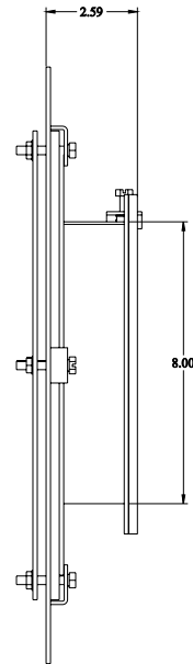
SIDE VIEW
