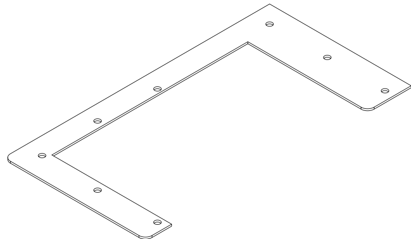
ISOMETRIC VIEW
