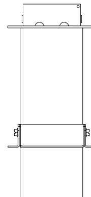
BOTTOM VIEW
