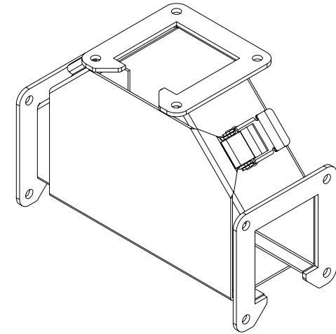
ISOMETRIC VIEW
