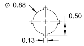
22.5mm Detail (1435M Series)
