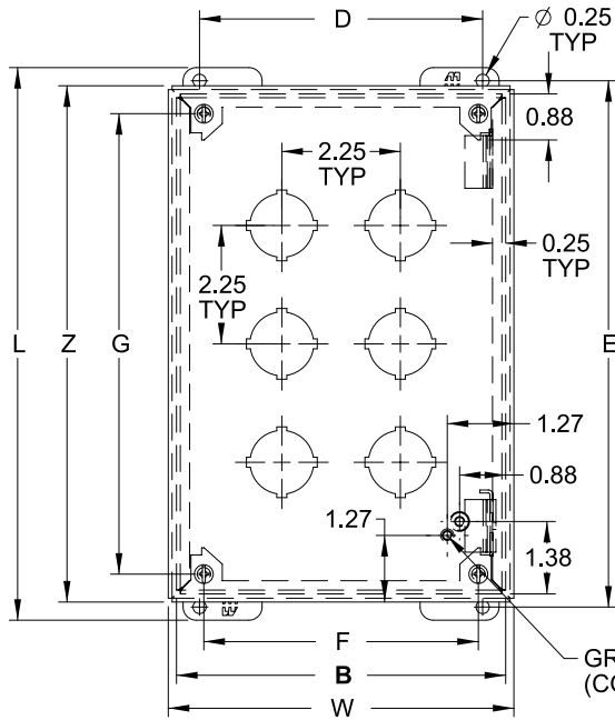
Front View Body Type F through S (Hinged)
