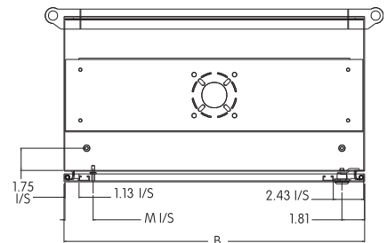
End View Section
