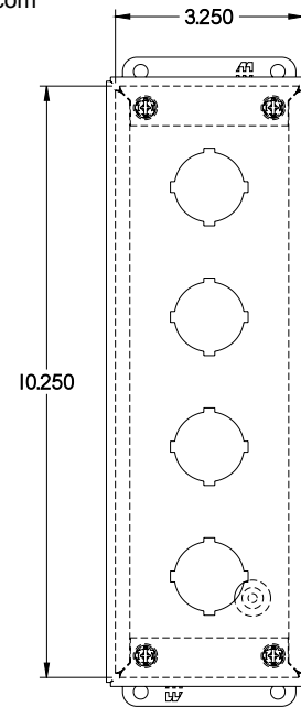
FRONT VIEW
