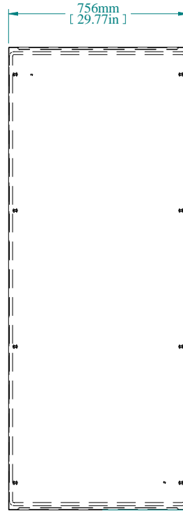
FRONT VIEW
