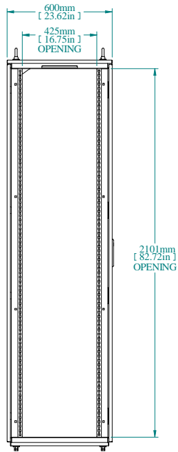
L.S. VIEW
