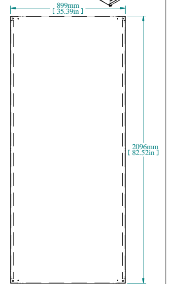
INNER PANEL
