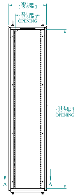
L.S. VIEW
