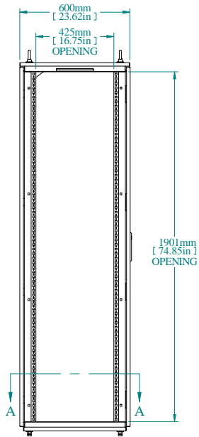
L.S. VIEW
