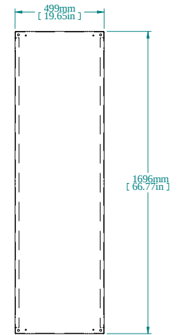
INNER PANEL
