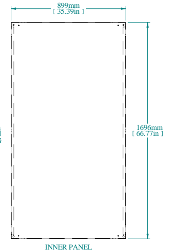
INNER PANEL
