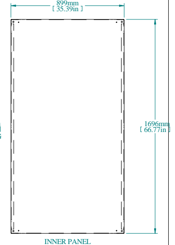
INNER PANEL
