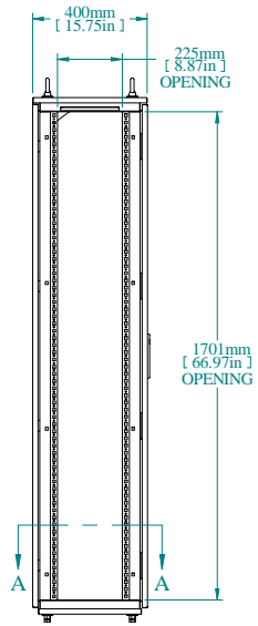
L.S. VIEW
