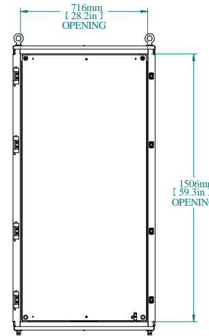
FRONT VIEW DOOR REMOVED
