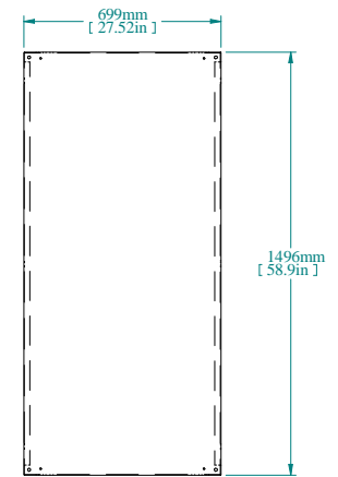
INNER PANEL
