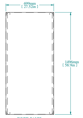
INNER PANEL
