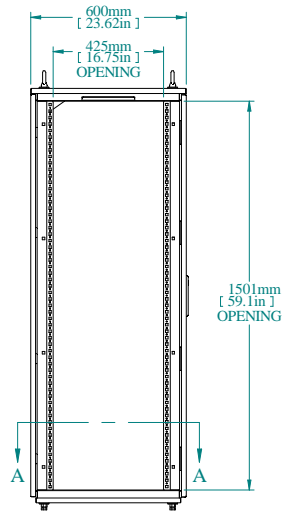
L.S. VIEW
