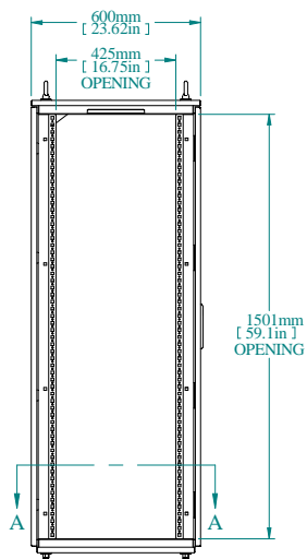
L.S. VIEW
