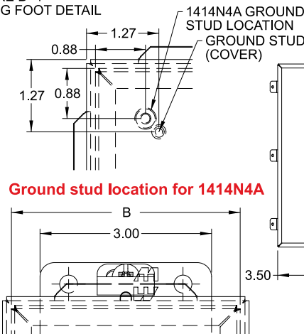
Mounting Detail When B= 4
