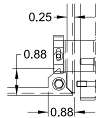
Hinge Detail
