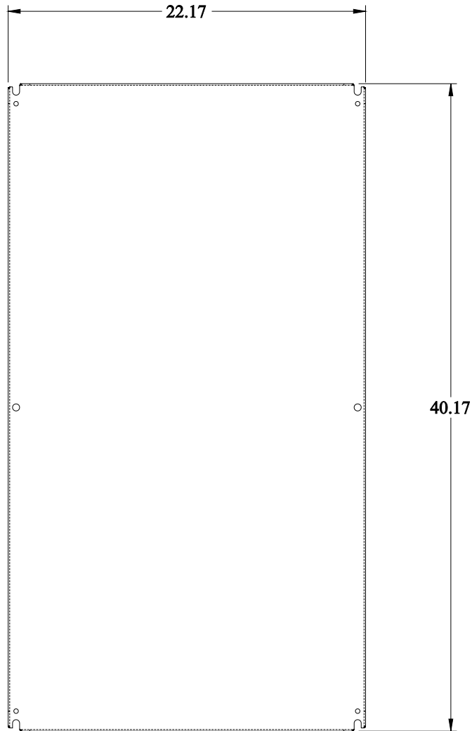
FRONT VIEW
