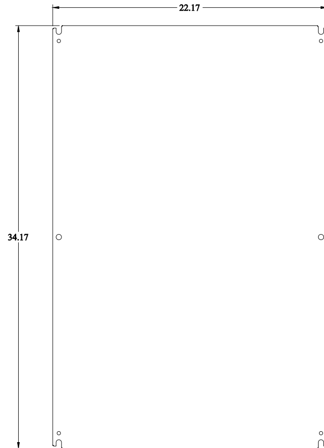
FRONT VIEW
