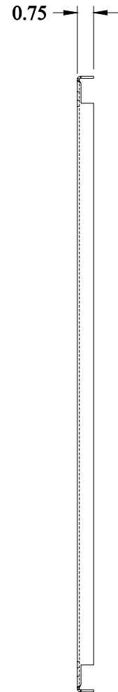
SIDE VIEW
