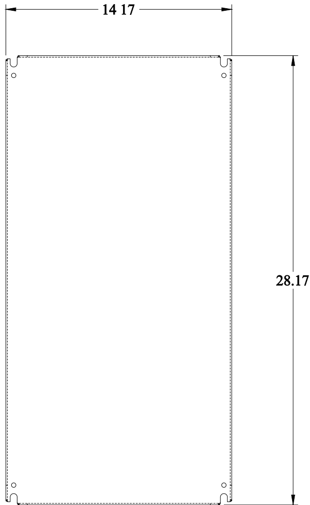
FRONT VIEW
