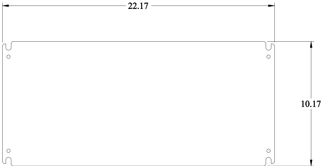
FRONT VIEW
