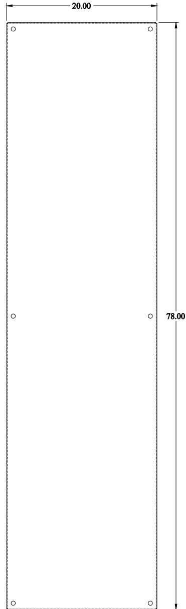
FRONT VIEW
