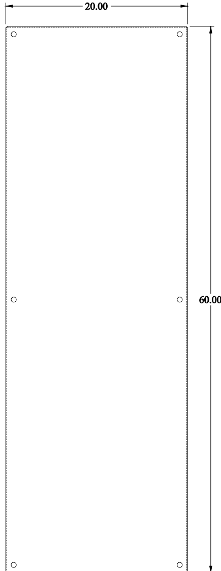
FRONT VIEW
