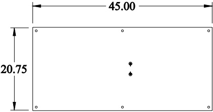
INNER PANEL
