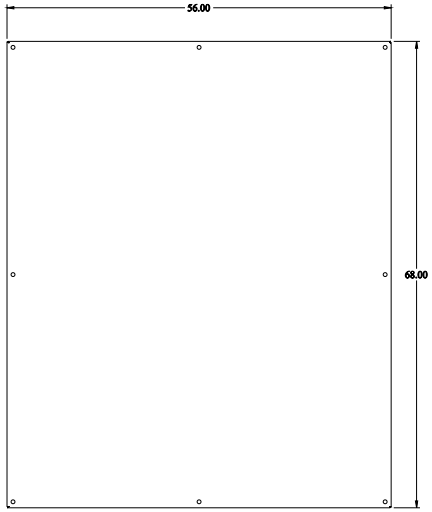
INNER PANEL
