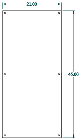
INNER PANEL
