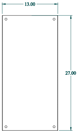
INNER PANEL
