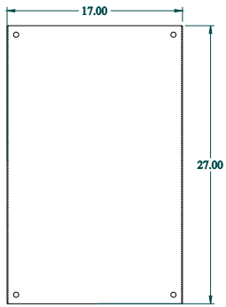
INNER PANEL
