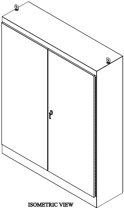
ISOMETRIC VIEW
