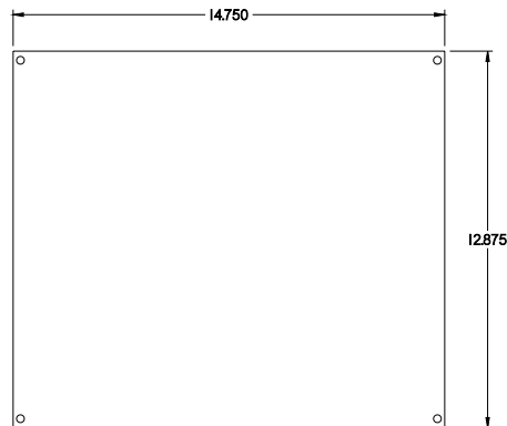
INNER PANEL
