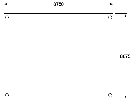
INNER PANEL
