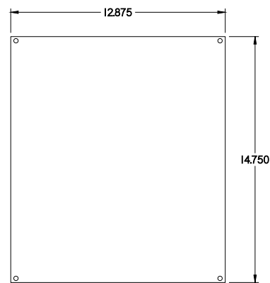
INNER PANEL
