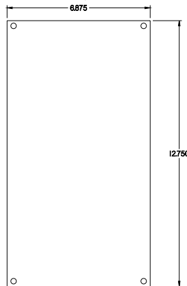
INNER PANEL
