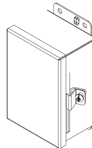
ISOMETRIC VIEW
