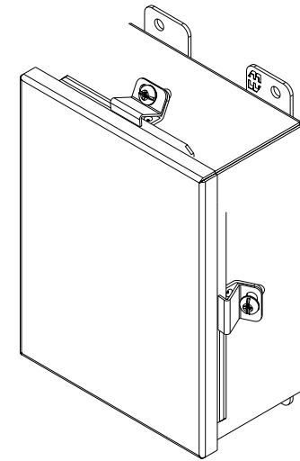
ISOMETRIC VIEW
