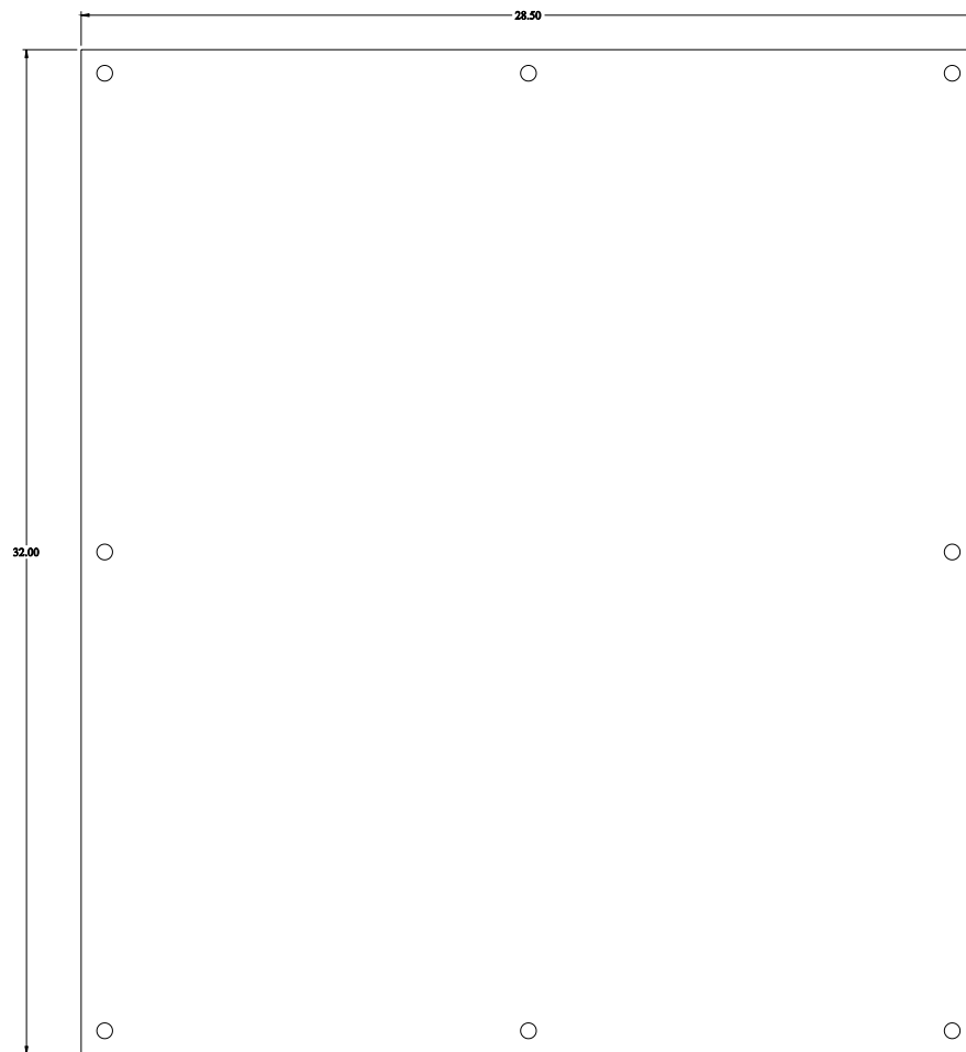
FRONT VIEW
