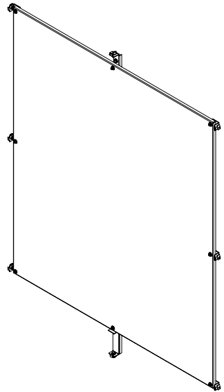
ISOMETRIC VIEW
