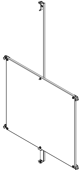
ISOMETRIC VIEW
