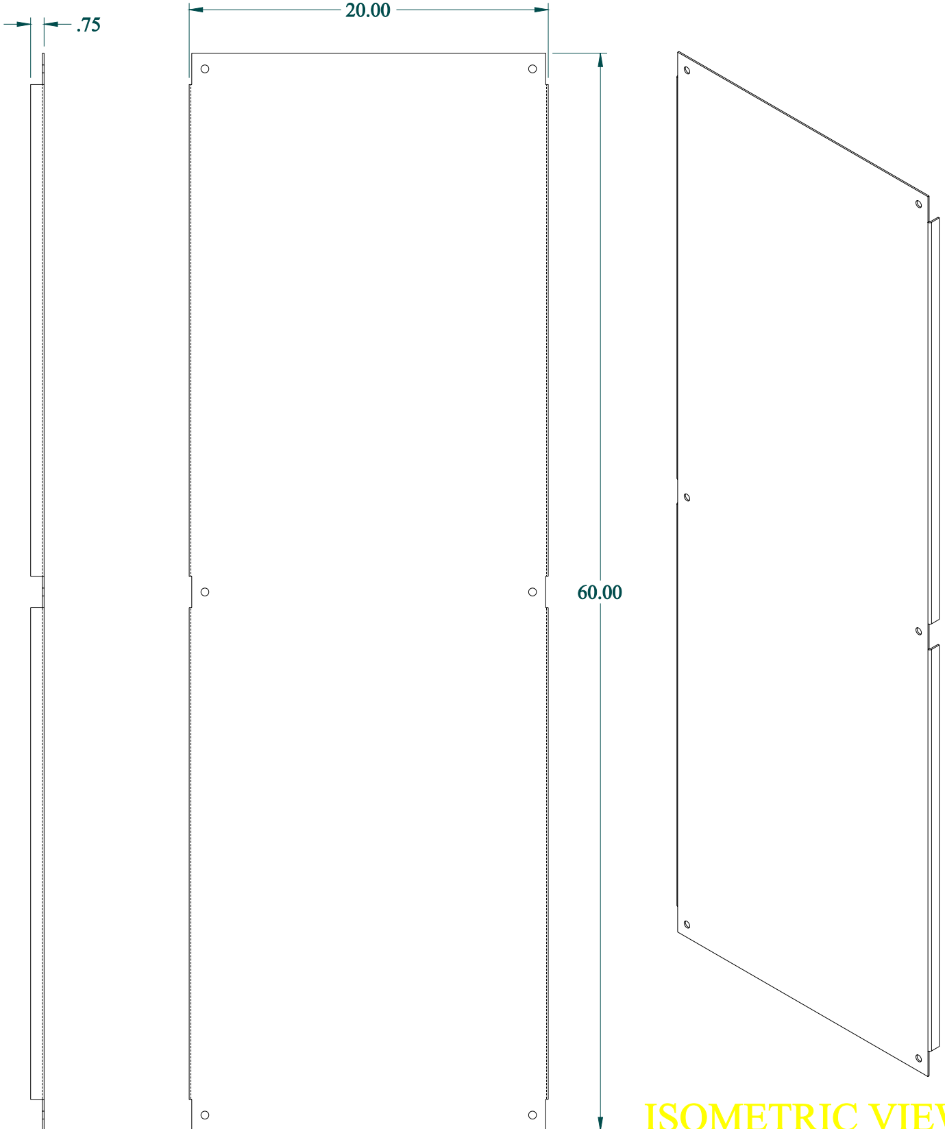
SIDE VIEW
