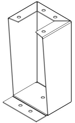
ISOMETRIC VIEW
